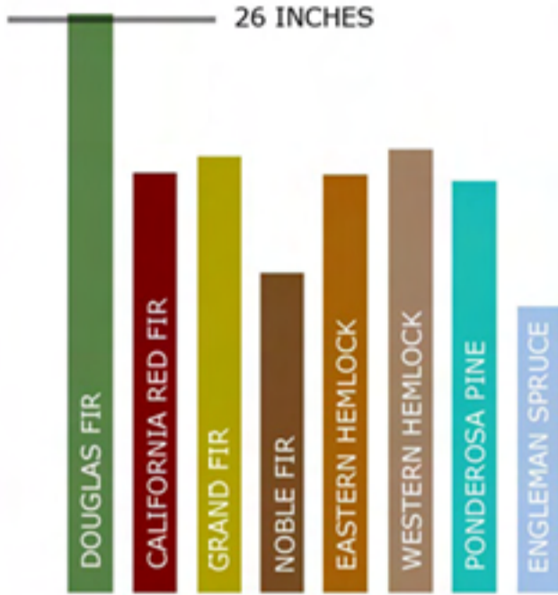
IMPACT BENDING
