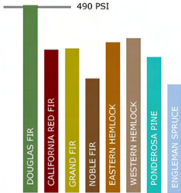
SIDE HARDNESS (PERPENDICULAR TO GRAIN)
