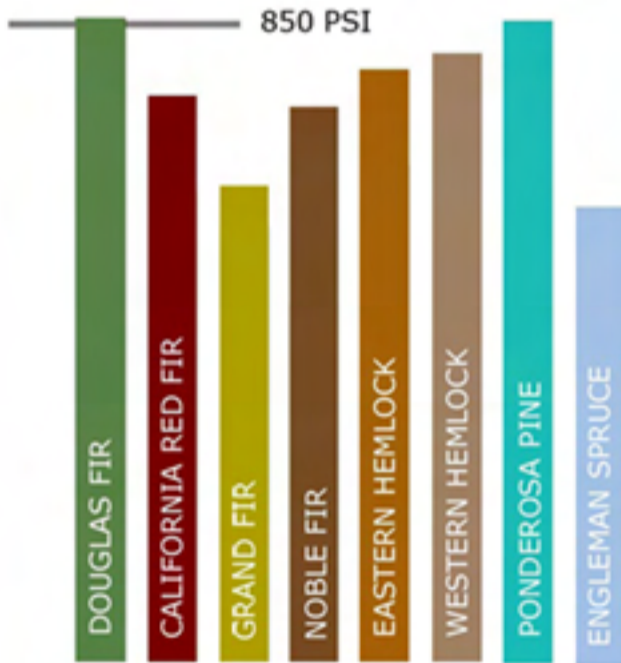
SHEARING STRENGTH
