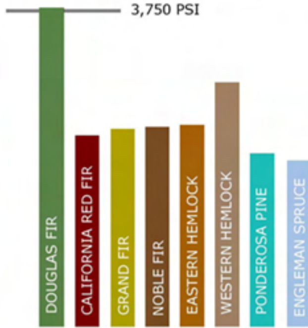
CRUSHING STRENGTH (PARALLEL TO GRAIN)
