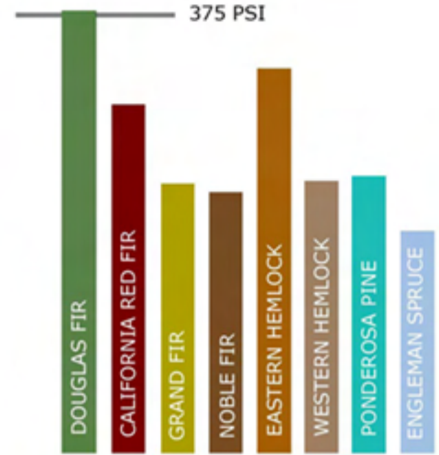
CRUSHING STRENGTH (PARALLEL TO GRAIN)
